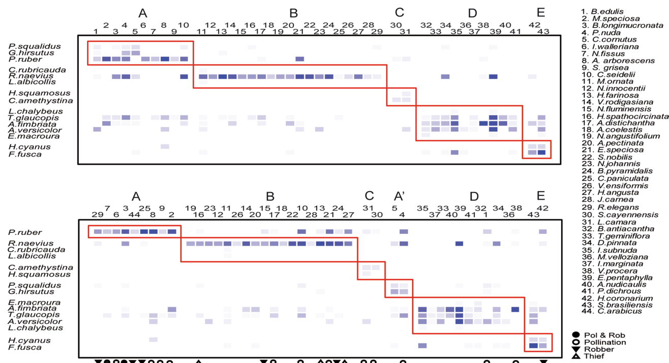
Fig. 3 Modules in the plant–hummingbird visitor network from Núcleo Pinguaba, southeastern Brazil. Top matrix Pollination network (PN) with only legitimate interactions, bottom matrix Visitation network (VN) also incorporated illegitimate interactions (nectar robbing and thieving). Uppercase letters above matrices denote identities of modules in the networks. Note that the original module (A) is separated into two modules (A, A′) when illegitimate visits are included.
