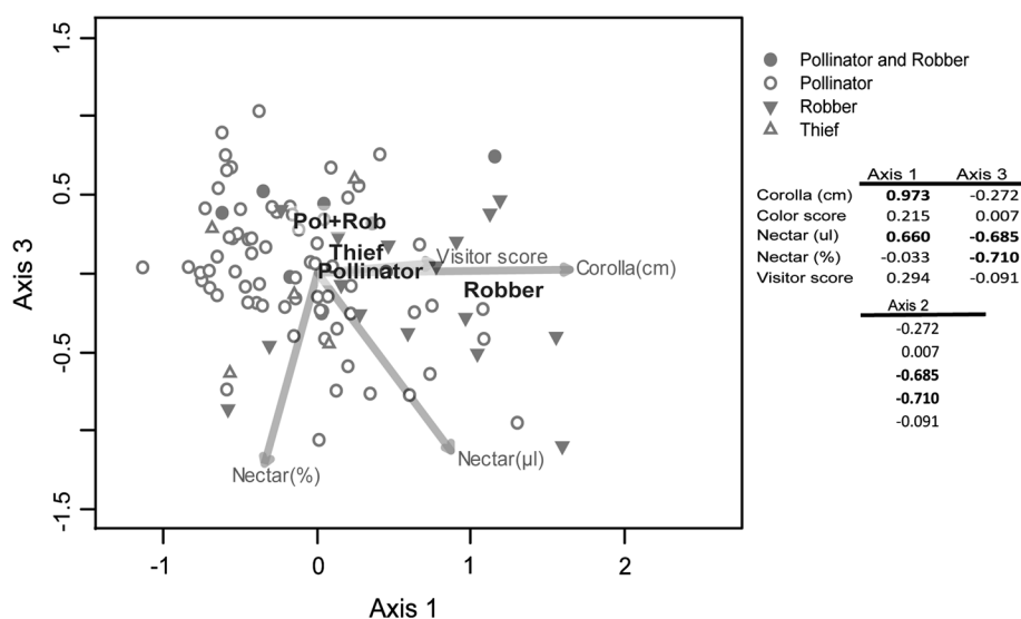
Fig. 1 Nonmetric multidimensional scaling (NMDS) of 97 plant species for which records on interaction with Phaethornis ruber were identified in our literature survey (stress level 10.19, r^2 = 0.93 ). Axis 1 was rotated according to floral corolla length and is shown together with axis 3. Right Pearson's correlation coefficient of the floral traits
